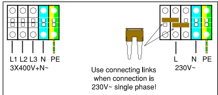
Three phase and single phase connection
